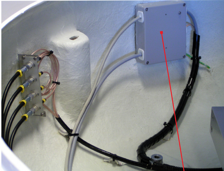
Connection of junction box inside radome
